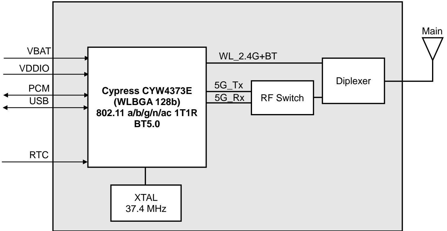
AW-CM467-USB-I BLOCK DIAGRAM
