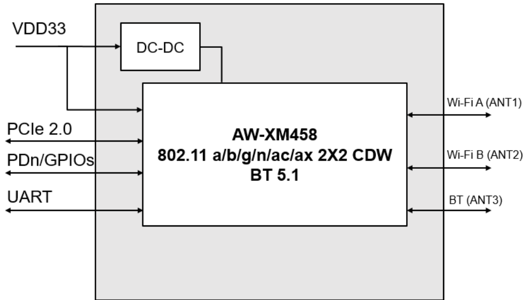
AW-XM458MA-PUR Block Diagram
