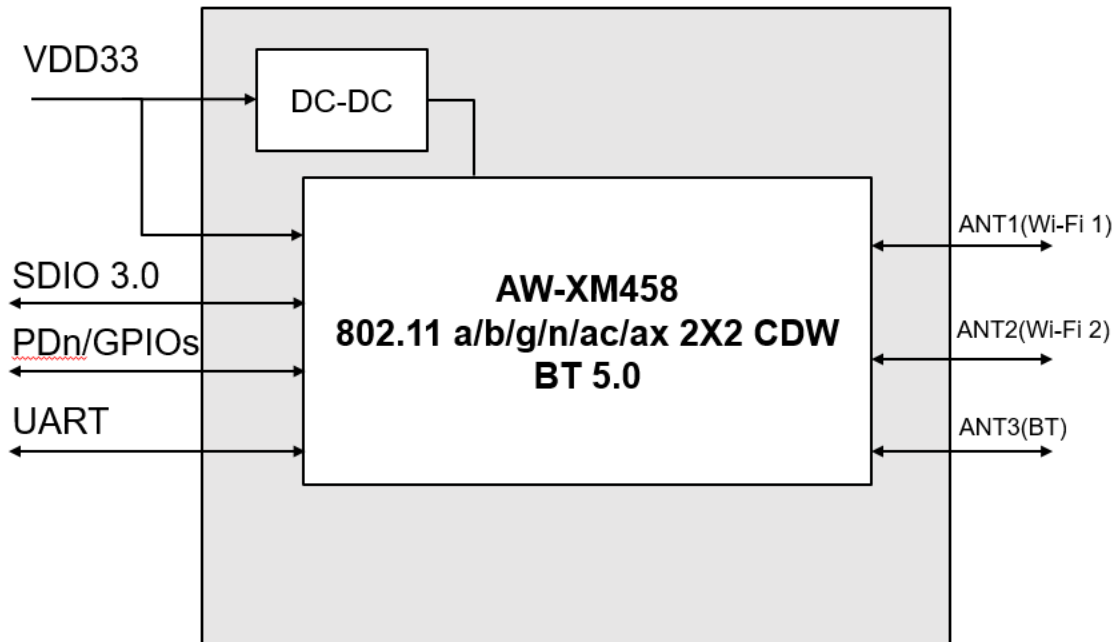
AW-XM458MA-SUR Block Diagram
